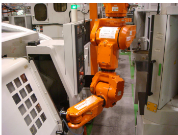
Inverted Mount 8 Axis Loader Nachi MR20
