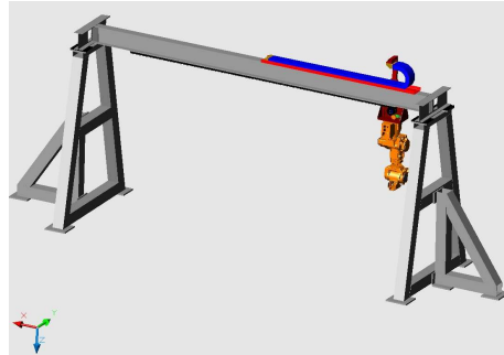
3D Layout Overhead Rail Robot Nachi MR20
