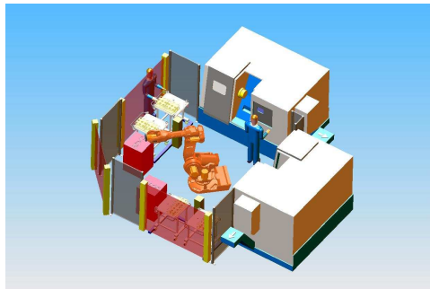
3D Concept 2 Machine Cell ABB IRB6600
