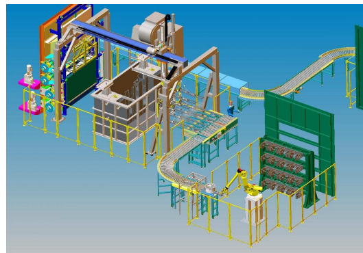
Quench tank gantry robot system
