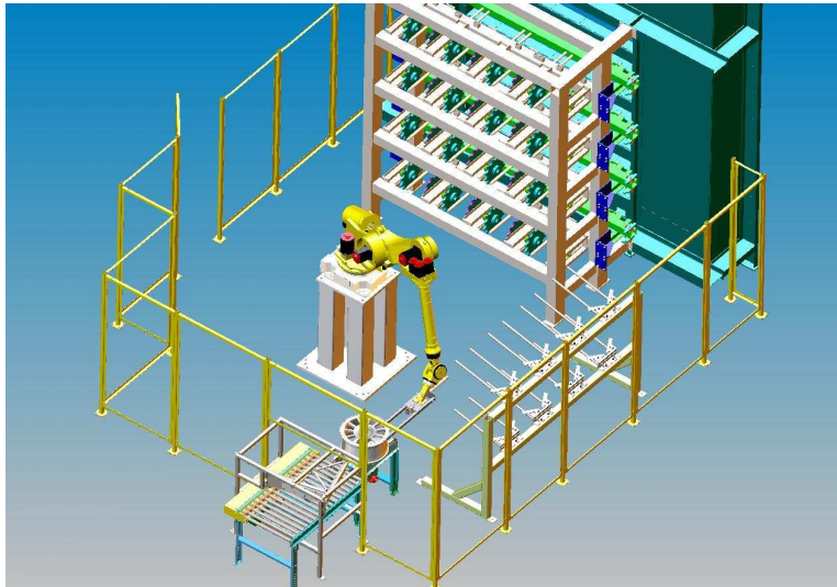
Complete Cells – Part Presentation, queuing and loading
