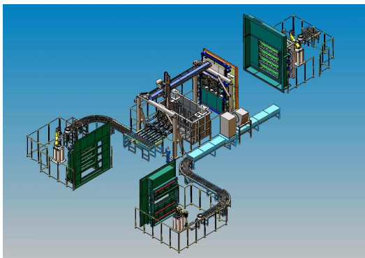
Furnace and oven handling system
