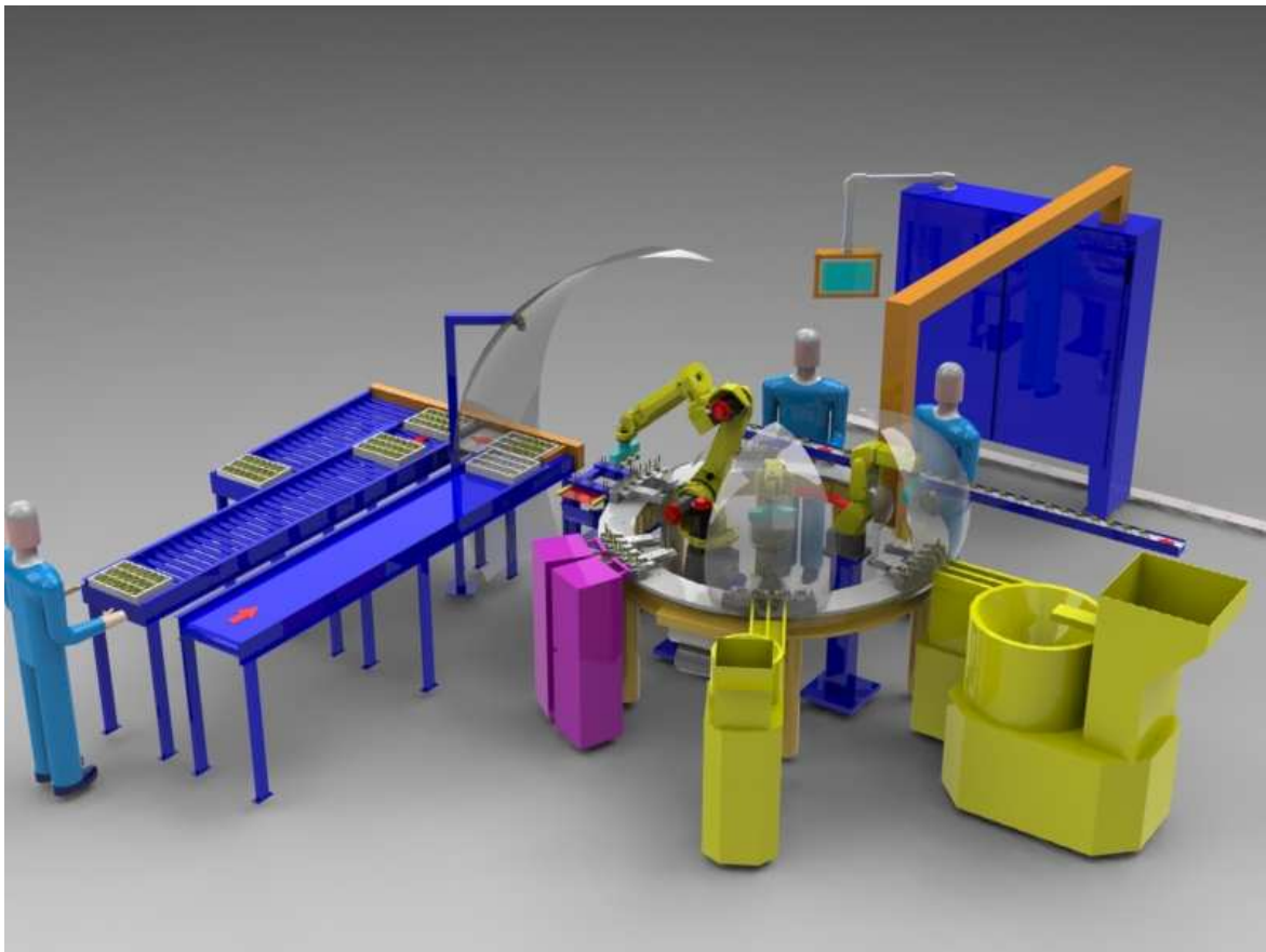
Six station dial machine with open center for ignition units
