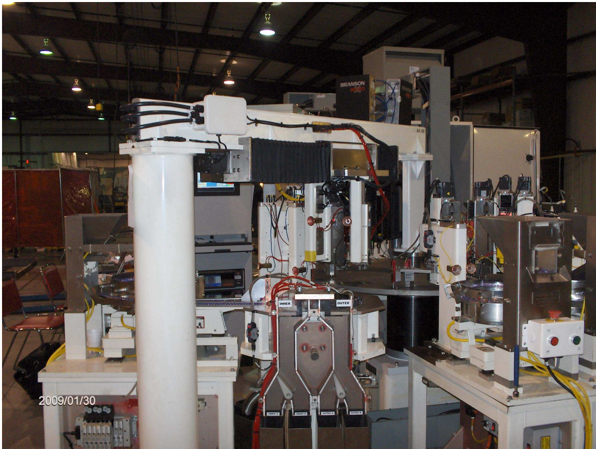
Twenty-four station dial machine for medical valves
