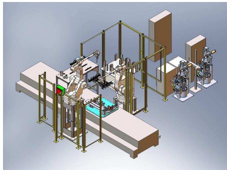
3D Layout Engine Sealing Line
