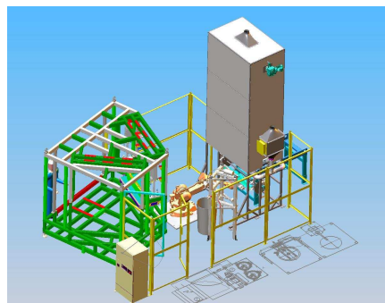
3D Layout 2K FIPG Automotive Lights With Cure Oven
