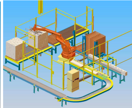
3D Layout '2 In, 2 Out' Case Cell ABB IRB640
