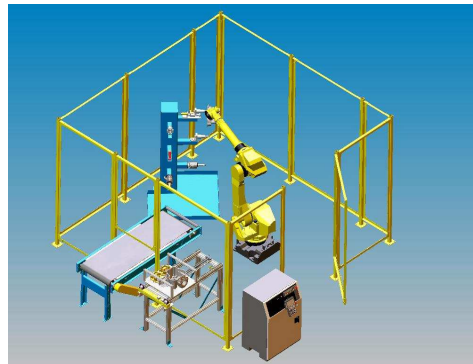
3D Layout Aluminum Casting Clean up Cell
