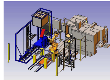
Machine L/UL with Deburring Robot with Vision
