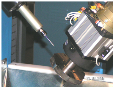
Deburring Pump Impellers Compliant Milling Tool
