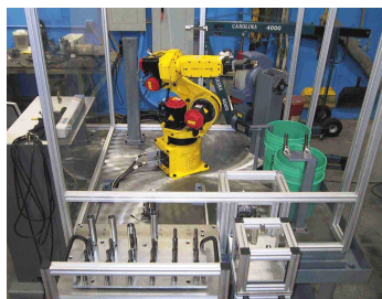
Deburring Rifle Receivers Fanuc M-16iA Drop in Cell
